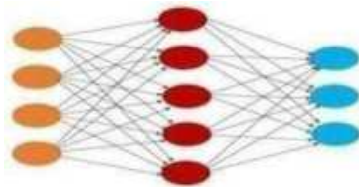
Fig 3.1 Neural networks
